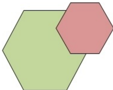
Figure 2: Valid Multipolygon
